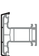
3316 416 grV Al cover cap mullion
