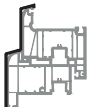
3319 507 grV Al cover cap sash-overhung
